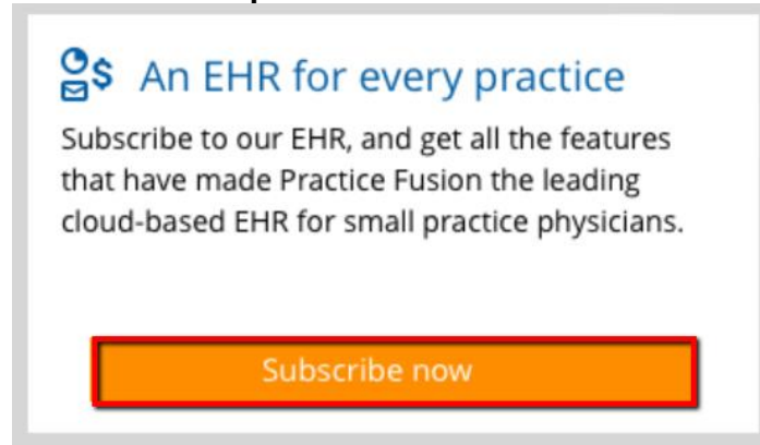
Graphic 4: Dashboard Tile
