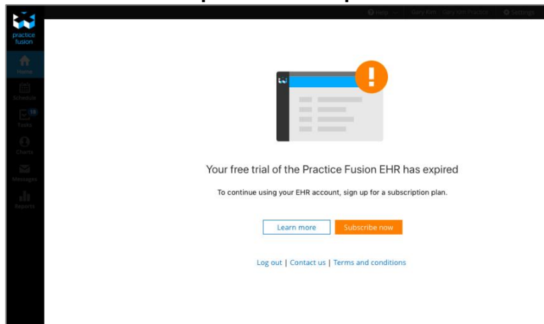
Graphic 3: Trial Expired
